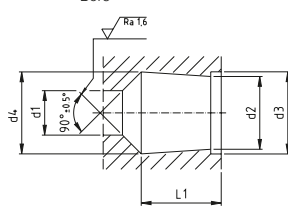
Bore (RVS 6-L/S / 8-S only) Bore (must align exactly)
